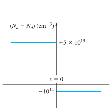
Figure P7.28 | Figure for Problem 7.28.
